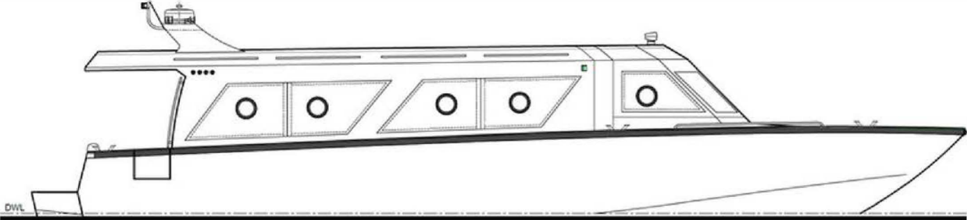
2 STBD PROFILE SCALE 1:80.00
