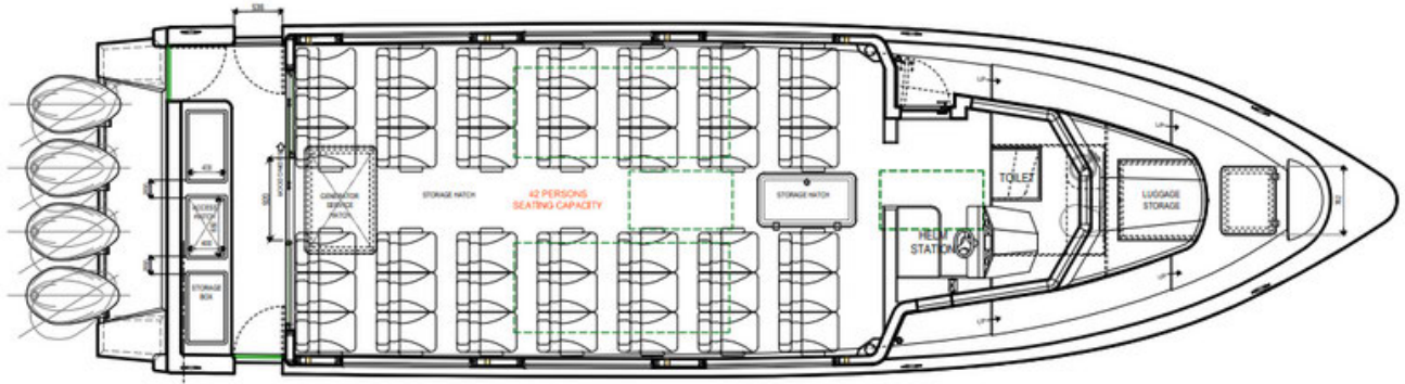
DECK PLAN
