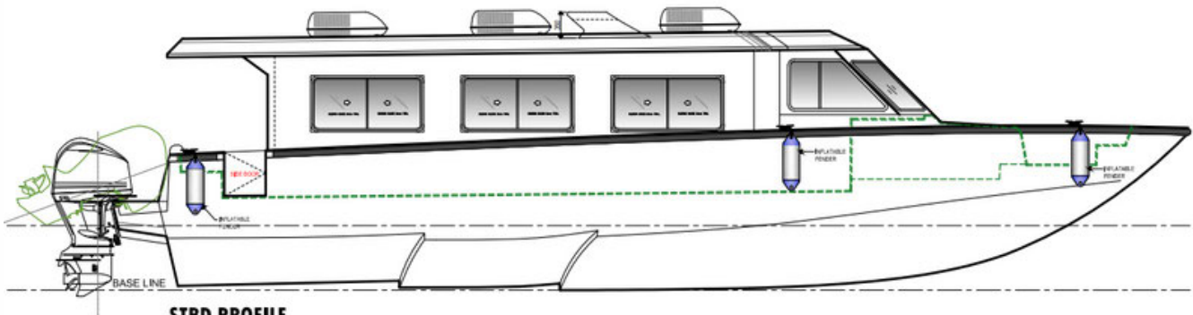
STBD PROFILE
