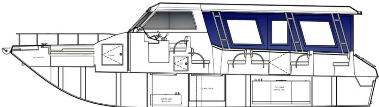
4 INBOARD SECTION (STBD) SCALE 1 : 50 M
