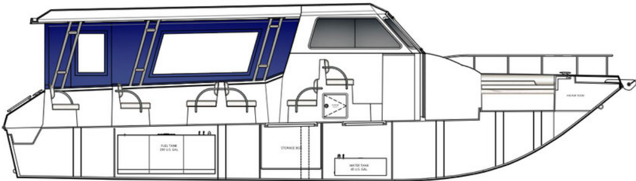
3 INBOARD SECTION (PS) SCALE 1 : 50 M
