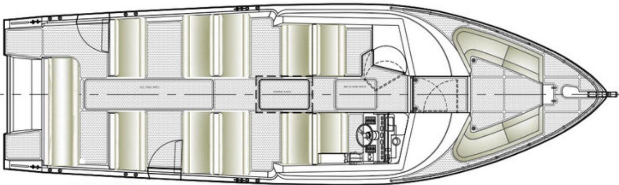
2 DECK PLAN SCALE 1 : 50 M
