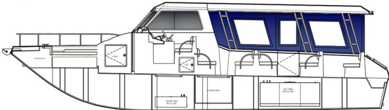
4 INBOARD SECTION (STBD) SCALE 1 : 50 M
