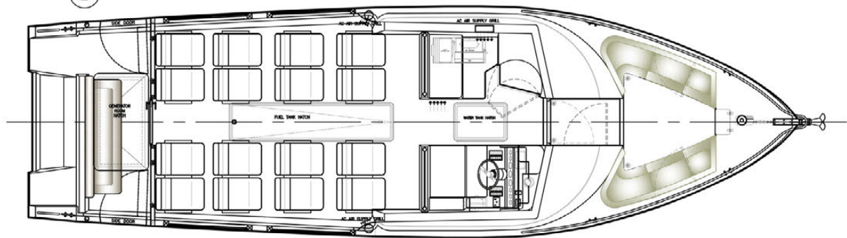
② DECK PLAN
