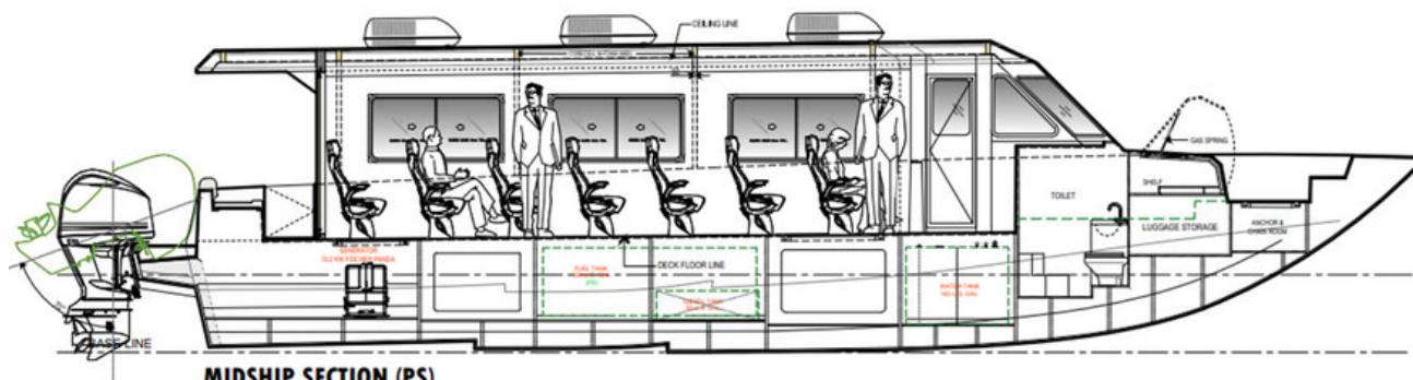
MIDSHIP SECTION (PS)
