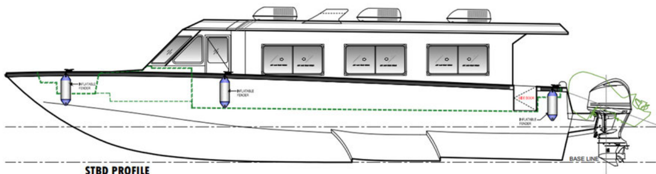
STBD PROFILE
