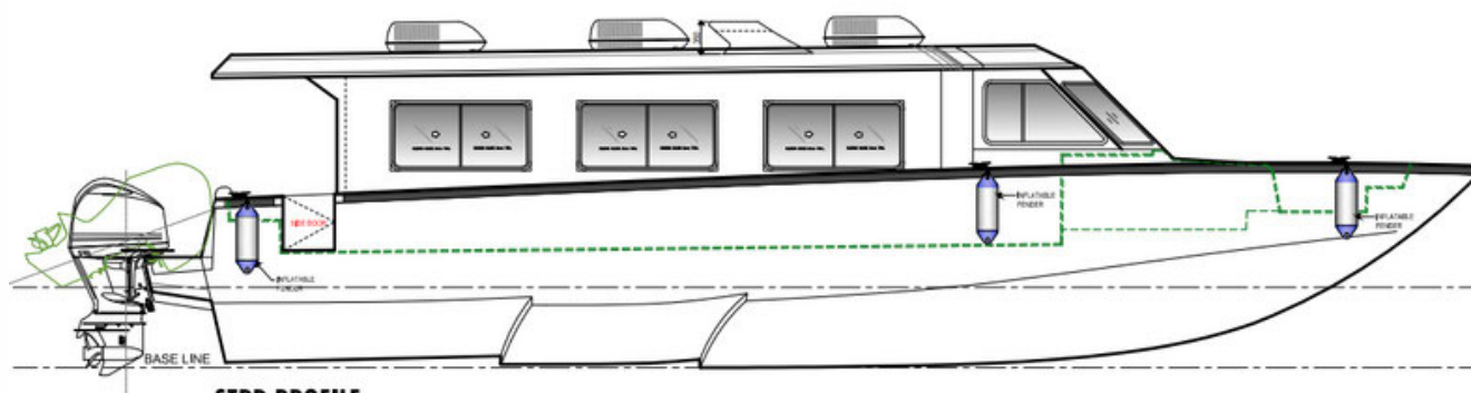
STBD PROFILE
