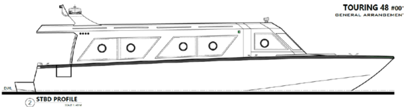
STBD PROFILE
