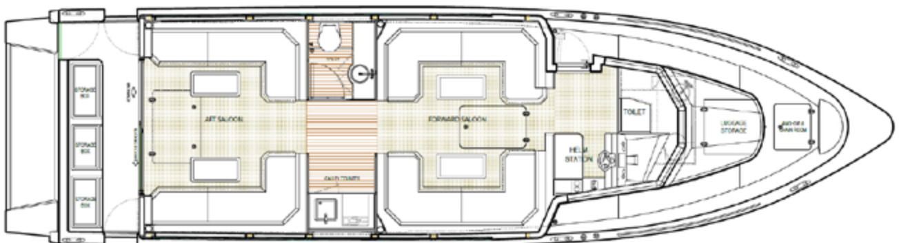
DECK PLAN
