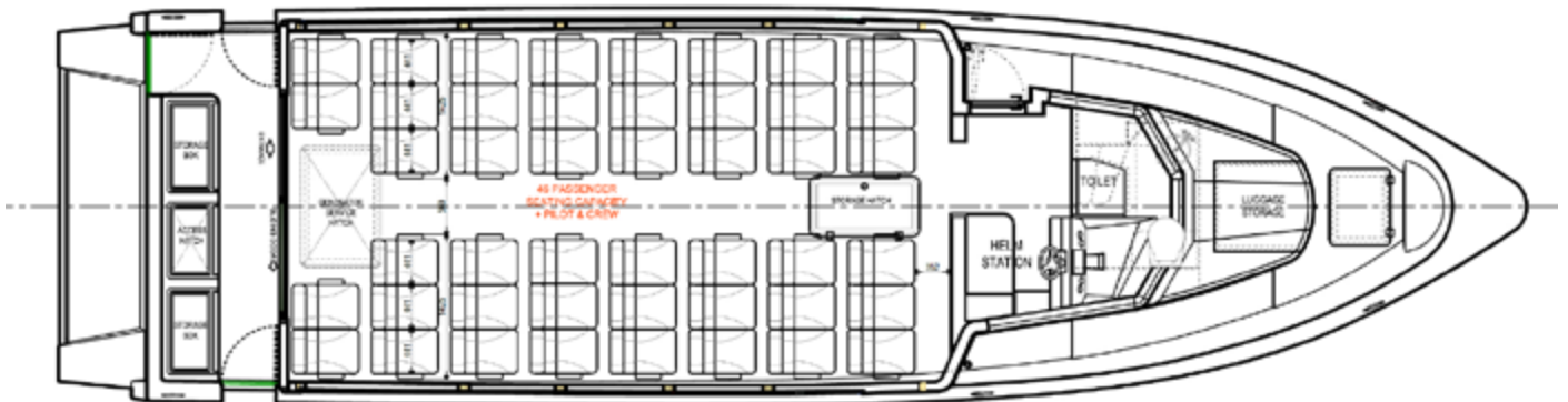
DECK PLAN (PASSENGER VERSION)
