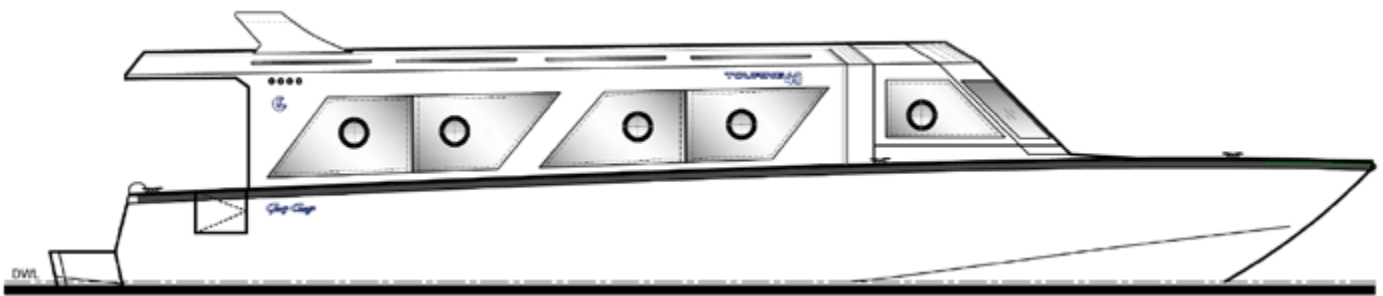
STBD PROFILE
