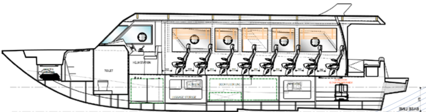
INBOARD SECTION (PS)
