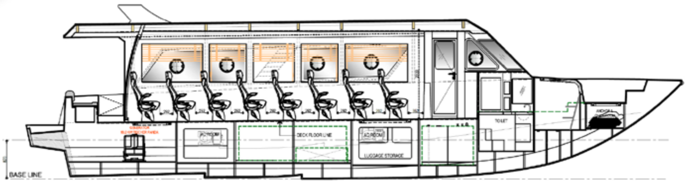
INBOARD SECTION (STBD)
