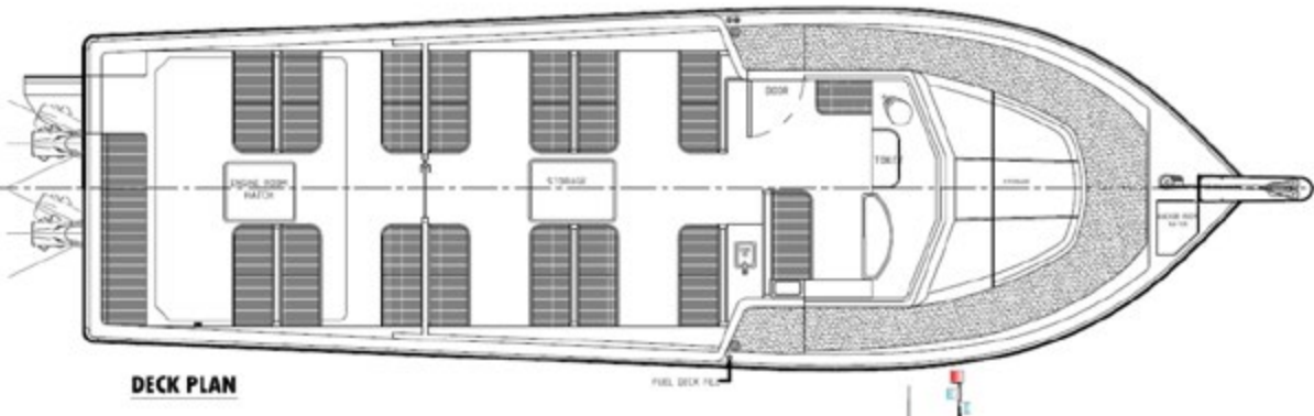
DECK PLAN
