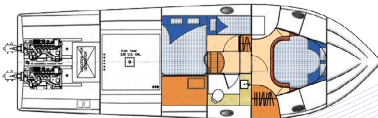
DECK PLAN
