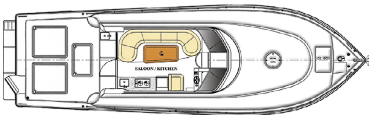
DECK PLAN
