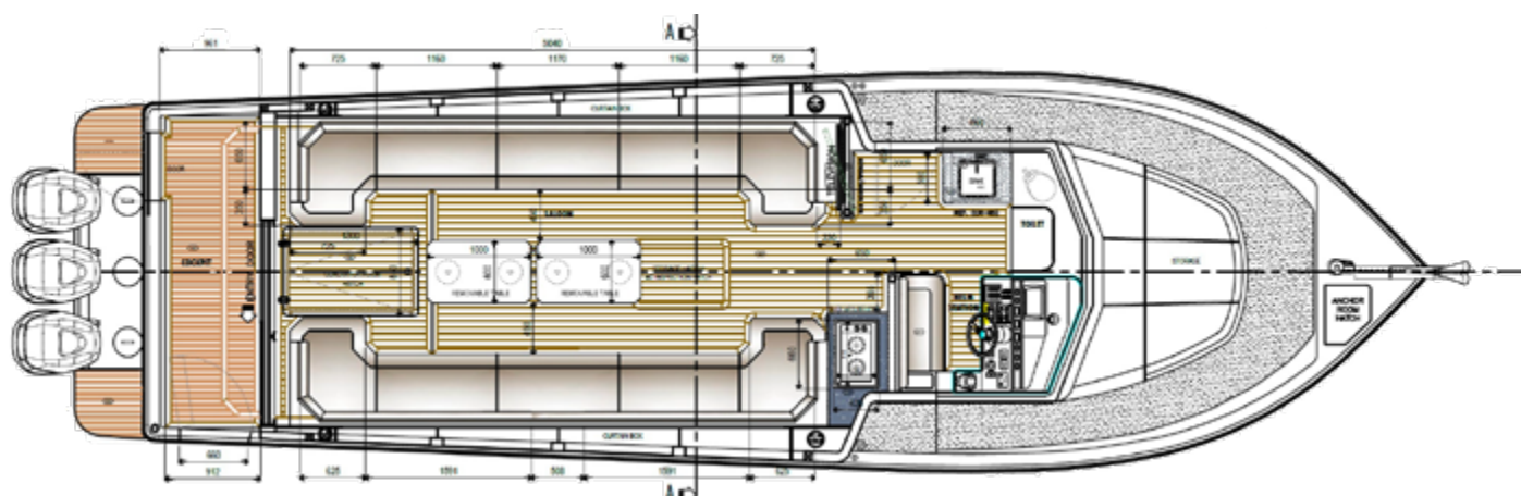
GENERAL ARRANGEMENT PLAN
