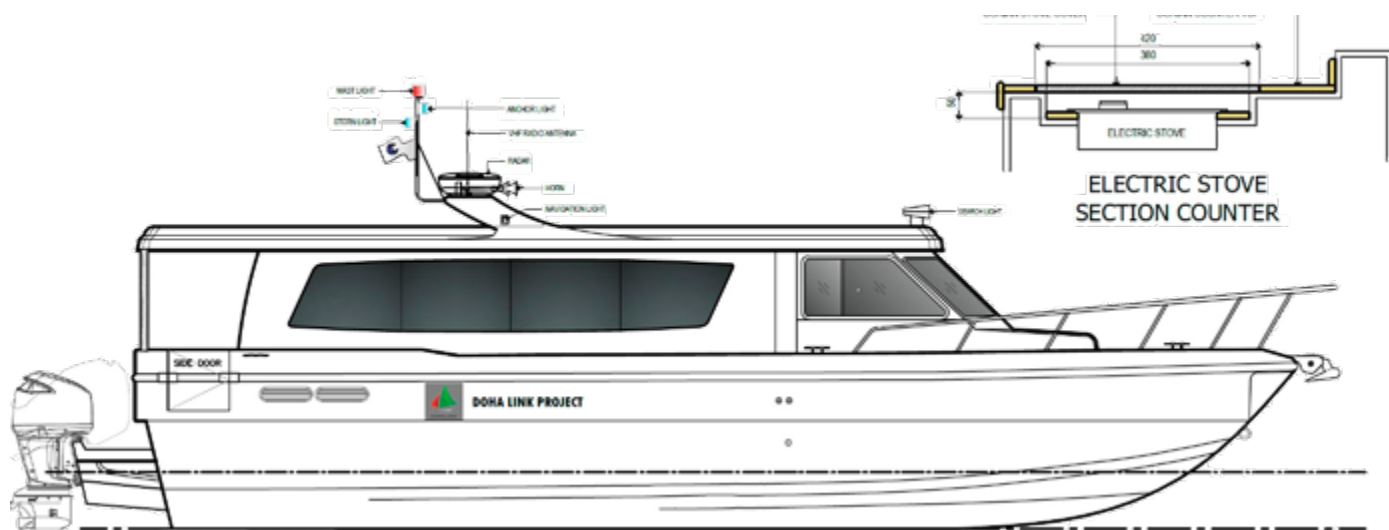
PROFILE (STBD)
