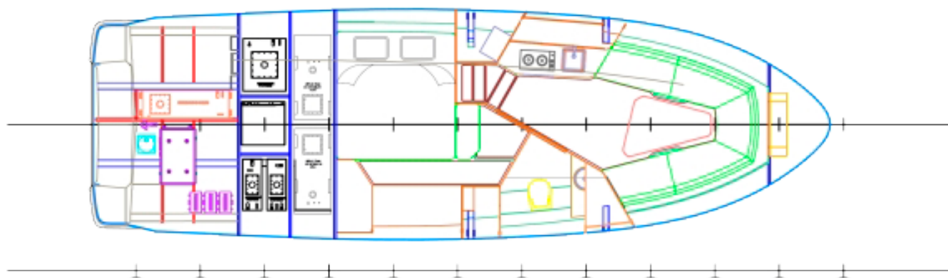
LOWER DECK
