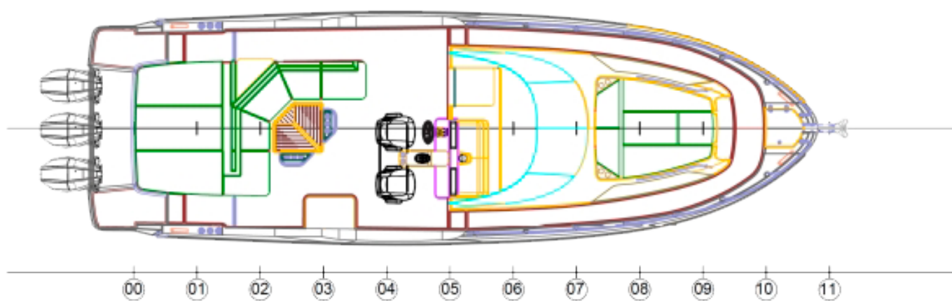
MAIN DECK
