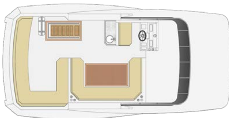
FLY-BRIDGE OPTION 1
