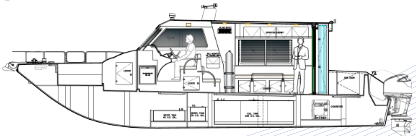
MIDSHIP SECTION (STBD)
