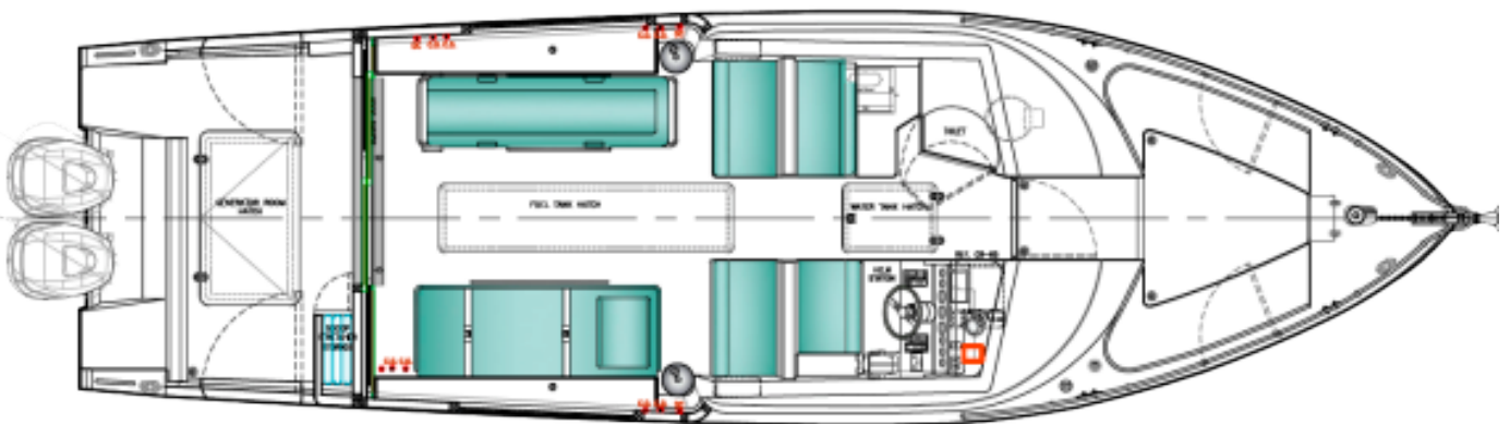
DECK PLAN
