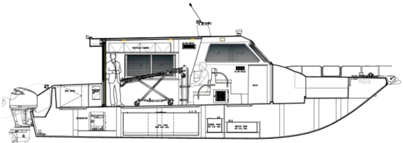
MIDSHIP SECTION (PS)
