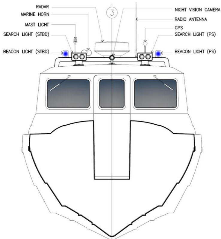
SECTION @ #3 SCALE 1:40 (VIEW FROM FWD)
