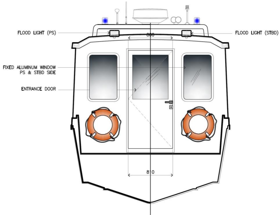
SECTION @ #10 SCALE 1:40 (VIEW FROM AFT)
